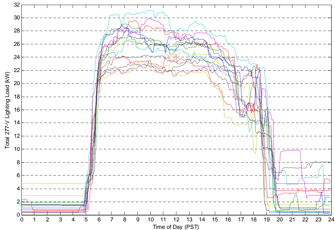
Figure 3.3. Building A Pre-Retrofit Weekday Load Profiles for Aug. 10 – Aug. 29, 2005
