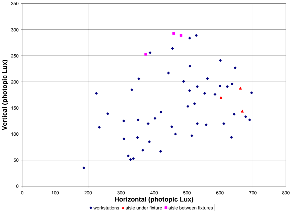
Figure 4.9. Building B - Pre-Retrofit Vertical vs. Horizontal Comparison (Photopic)
