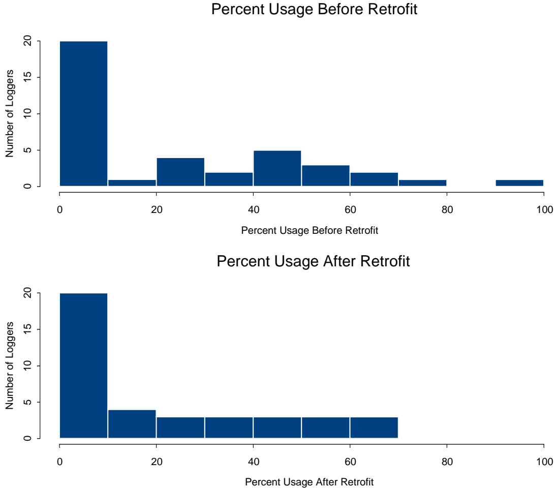
Figure 3.12. Building A - Task Light Usage as a Percentage of Business Hours Before and After Retrofit
