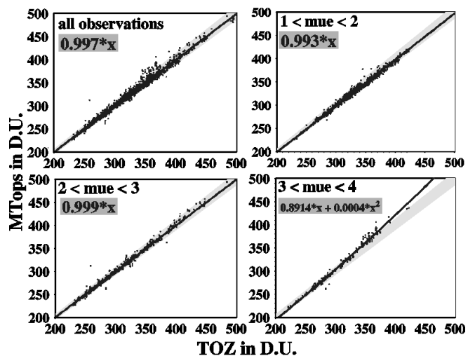
Figure 2a-d. Comparison between MTops and Dobson/Dobson-normalized Brewer total ozone in different sun elevation ranges. Top left : all observations; top right: 1 < \mu < 2 ; bottom left: 2 < \mu < 3 ; bottom right: \mu > 3 . \pm 3\% difference is marked by the grey area, the linear regression fit by the solid line.
