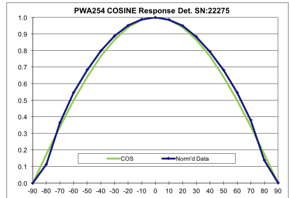
Fig. 3. Cosine Response
