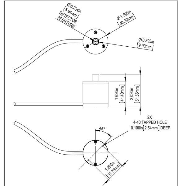
Liquid Light Guide Sensor 2153
