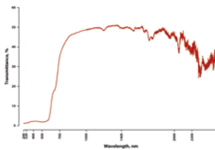
Figure: Transmittance Spectrum of the Test Fabric
