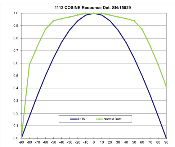
Fig. 3. Transverse Cosine Response
